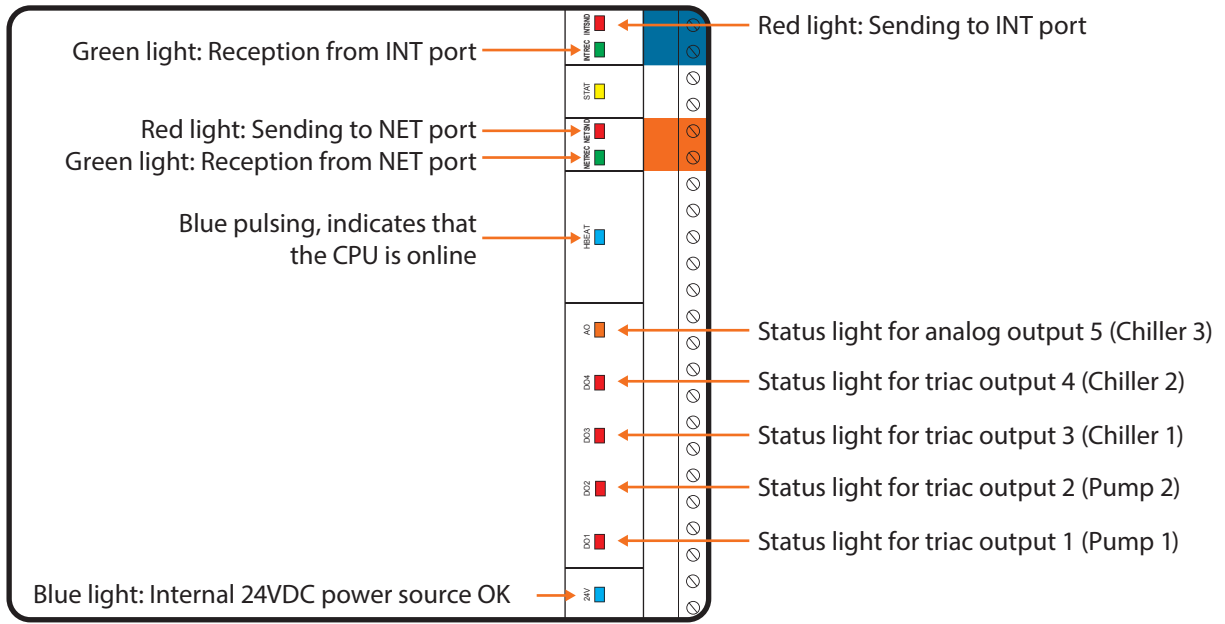
Figure 2 - LEDs Identification
